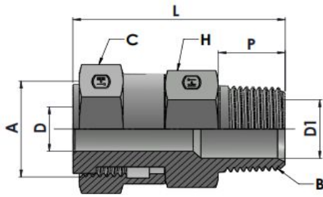
XXHTFS6505-00-00 Series MP-FSS STRAIGHT
