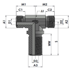
XXHTFS2703-00-00 Series MFS-MFS-MFS-MFS BULKHEAD TEE
