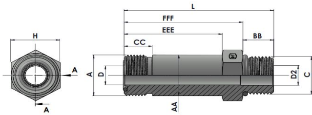
XXHTFS6400-L-00-00-O Series MFS-MORB STRAIGHT LONG
