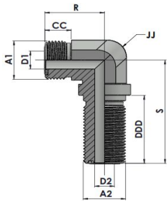
XXHTFS2701-00-00 Series MFS-MFS BULKHEAD 90° ELBOW
