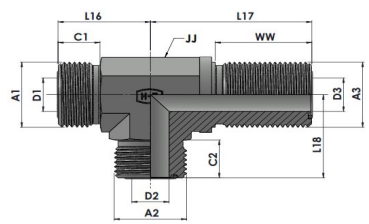
XXHTFS2704-00-00 Series MFS-MFS-MFS-MFS BULKHEAD RUN TEE
