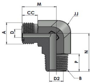
XXHTFS2501-00-00 Series MFS-MP 90° ELBOW
