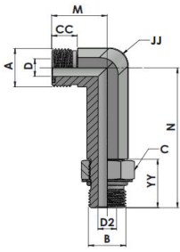
XXHTFS6801-L-00-00 Series MFS-MAORB 90° ELBOW LONG
