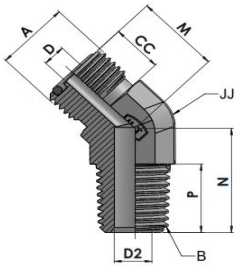
XXHTFS2503-00-00 Series MFS-MP 45° ELBOW
