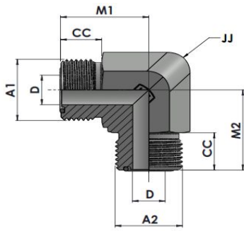
XXHTFS2500-00-00 Series MFS-MFS 90° ELBOW
