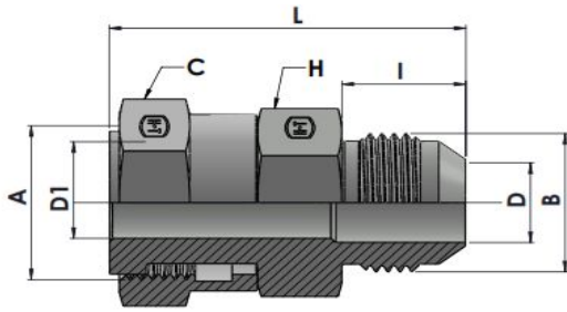
XXHTFS6504-00-00 Series FFSS-MJ STRAIGHT
