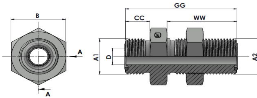
XXHTFS2700-00-00 Series MFS-MFS BULKHEAD UNION
