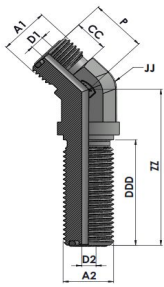
XXHTFS2702-00-00 Series MFS-MFS BULKHEAD 45° ELBOW
