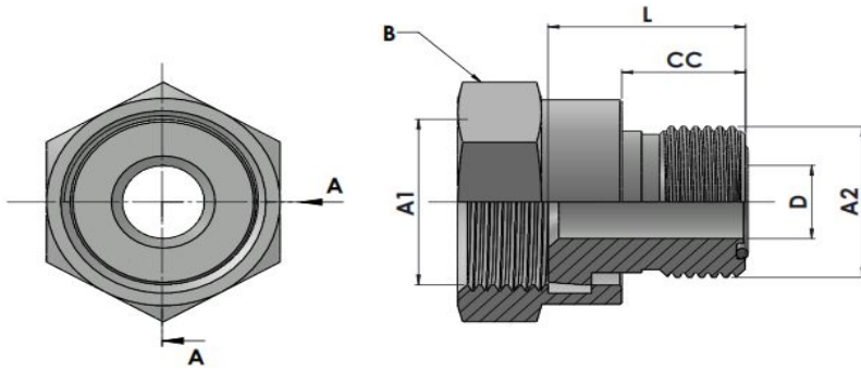
XXHTFS2406-00-00 Series FFS-MFS Straight
